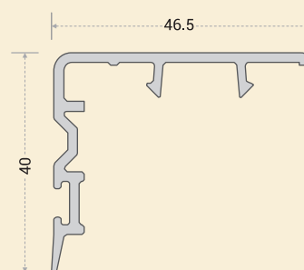
AW-1302 : SUPER SASH INTER LOCK
