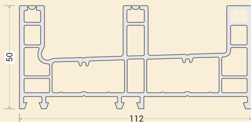
AW-1003 : S/W-3 TRACK FRAME
