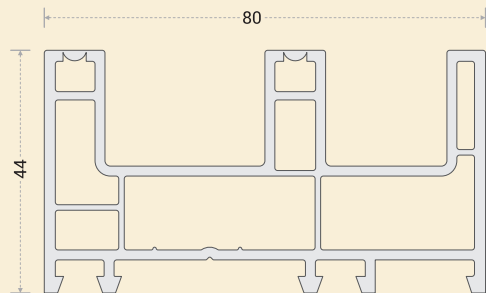
AW-1004 : 2.5 TRACK 80 MM
