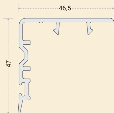
AW-1303: S/D INTER LOCK
