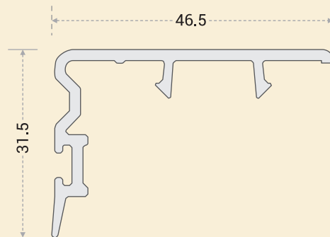
AW-1301: S/W INTER LOCK
