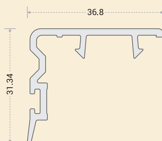
AW-1304 : S/W INTER LOCK
