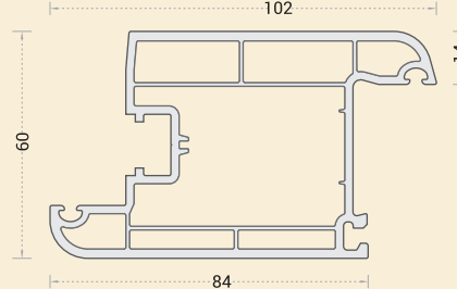
AW-2103 : C/D Z- SASH
