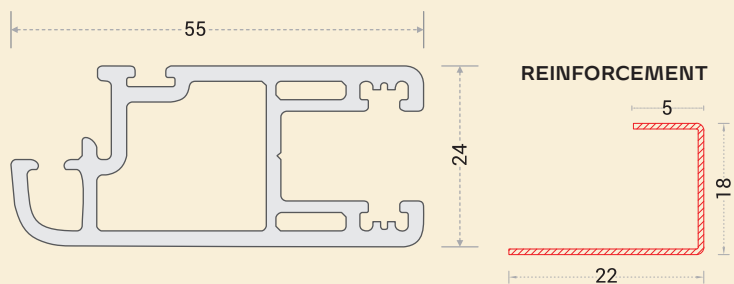
AW-1303: S/W - MESH
