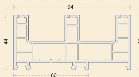
AW-1005 : 3 TRACK FRAME 94 MM
