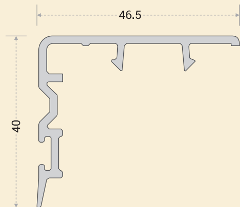
AW-1302: S/W BIG INTER LOCK
