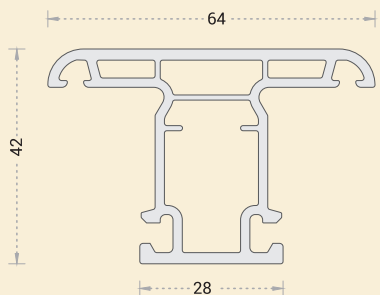
AW-3001 : SMALL CASEMENT SASH MULLION
