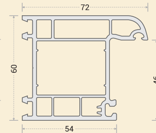
AW-2002 : C/D OF
