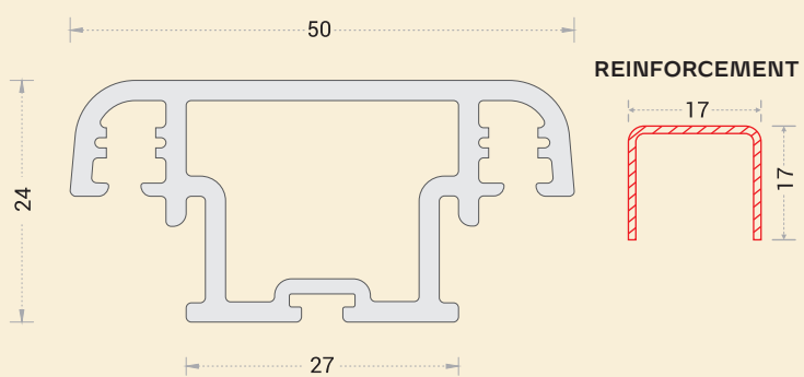
AW-1205: MESH MULLION
