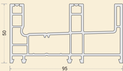
AW-1002 : 2.5 TRACK FRAME
