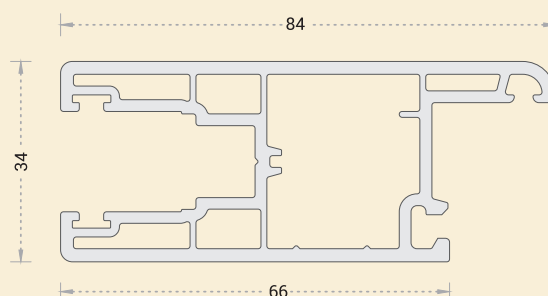
AW-1105 : S/D SASH 80 SERIES
